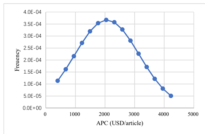
FIGURE 6 | Normal distribution of the APC of China biomedical journals both indexed by DOAJ and PMC
