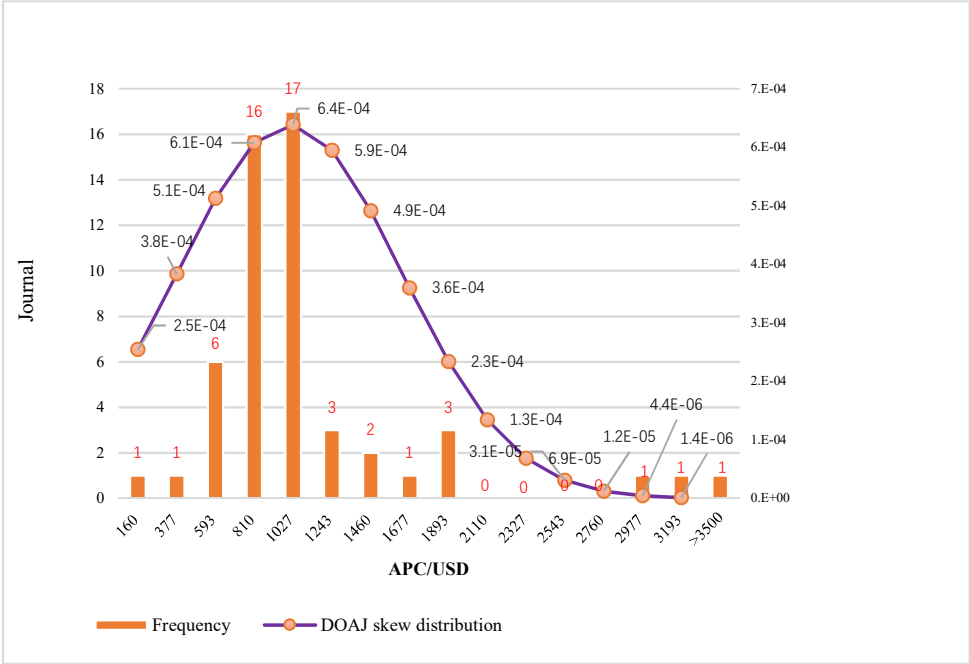
FIGURE 3 | Skew distribution of the APC of China’s biomedical journals indexed in DOAJ
